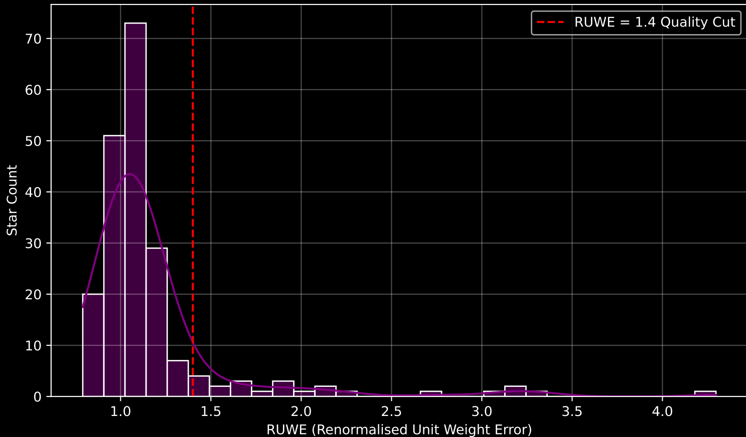
GAPOGEE DR17 Field [235+42_MGA] RUWE Distribution (n= 203)
