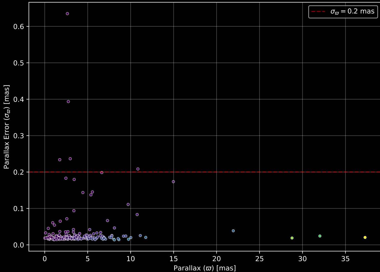
APOGEE DR17 Field: [235+42_MGA] Parallax Quality (n= 216)
