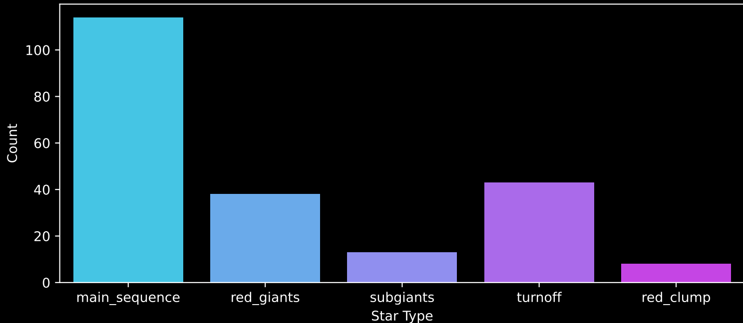
APOGEE DR17 Field: [235+42_MGA] Count plot of Star Type
