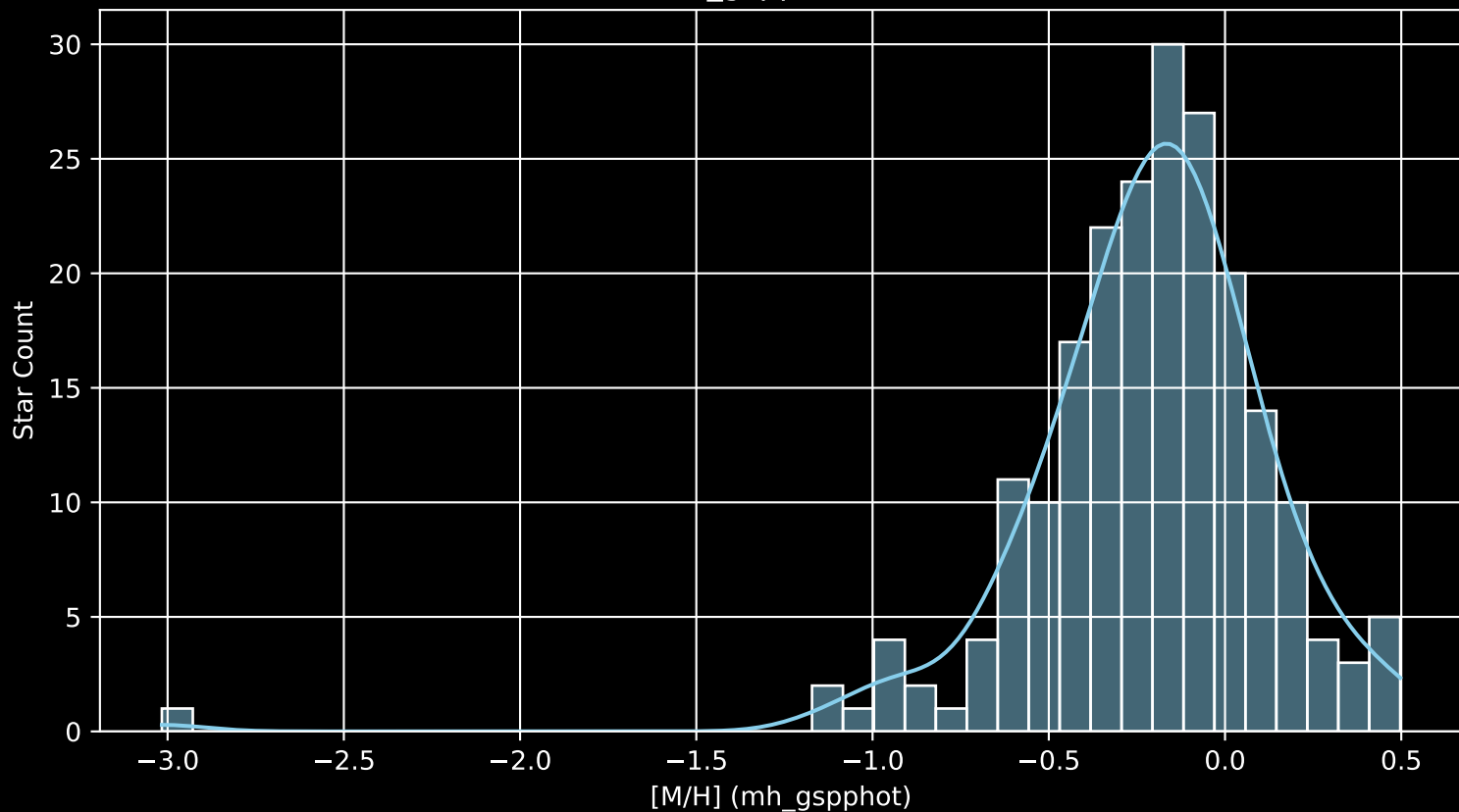
APOGEE DR17 Field: [235+42_MGA [M/H] (mh_gspphot) (n= 212)
