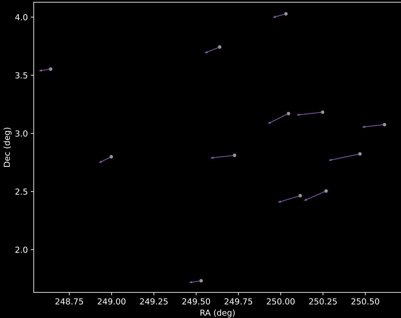
APOGEE DR17 Cluster 8 Proper Motion Vectors (n=12)
