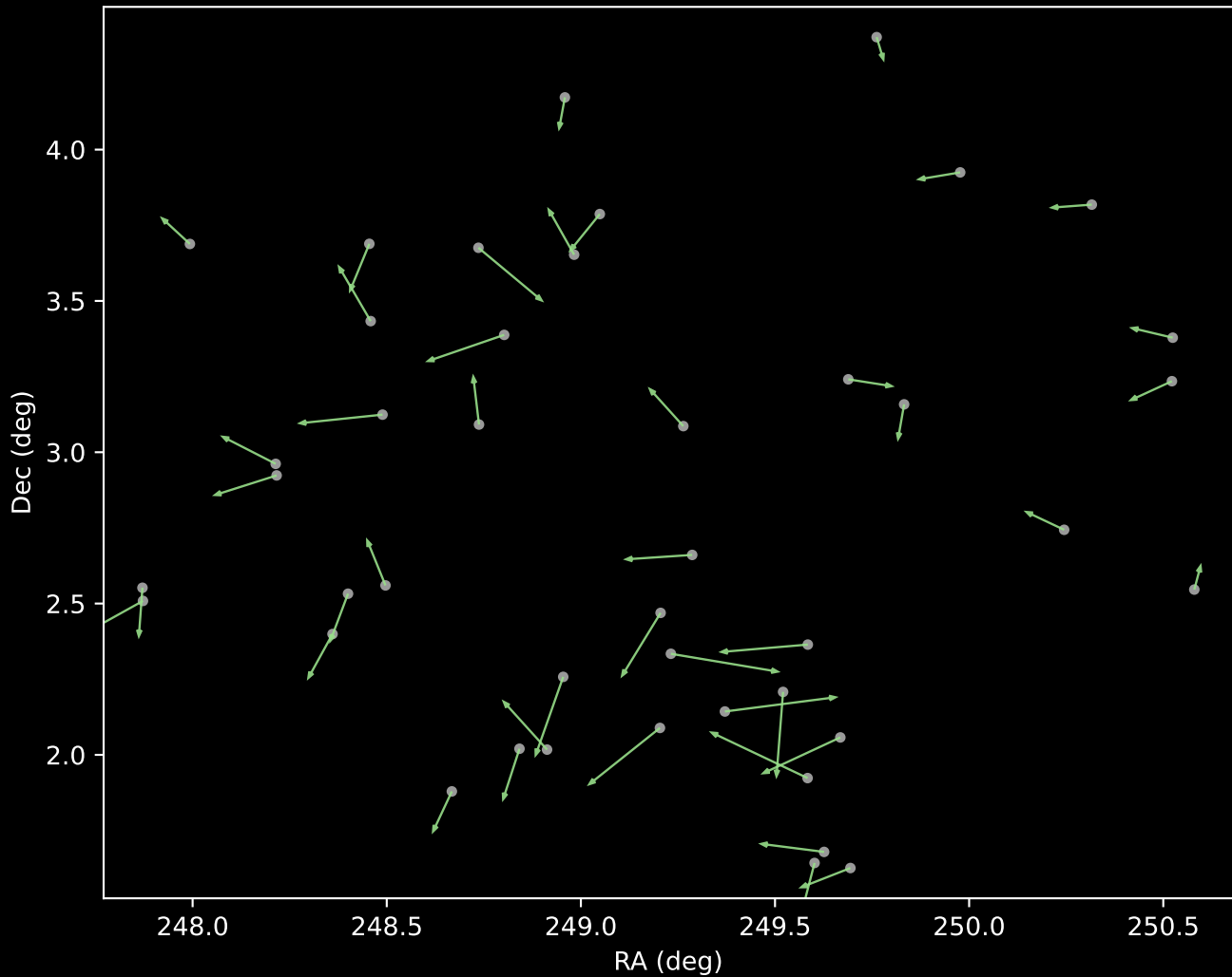
APOGEE DR17 Cluster 5 Proper Motion Vectors (n=43)
