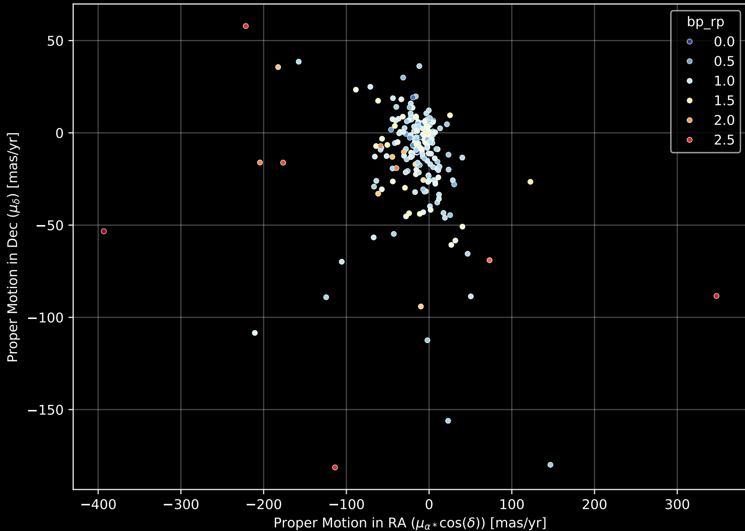
APOGEE DR17 Field: [235+42_MGA] Proper Motion Diagram (n= 216)
